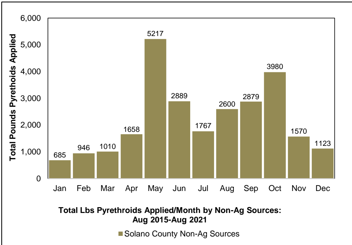
Total pounds of pyrethroid pesticides applied by non-agricultural pesticide applicators per month in Solano County: August 2015 – August 2021.
