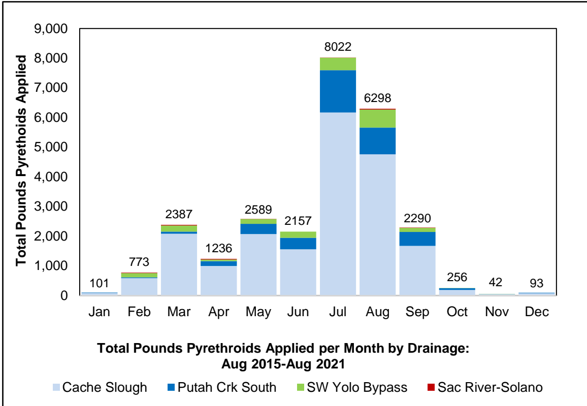
Total pounds of pyrethroid pesticides applied by agriculture per month in drainages relevant to the Ulatis Creek at Brown Road monitoring site: August 2015 – August 2021.
